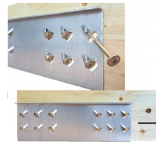
Fig 3b1: Note how the screws are installed into the guided slots at an angle. Below image: Steel Strong-Portal shoe with all screws installed. Example shows LH column, arrow indicates direction to RH column
