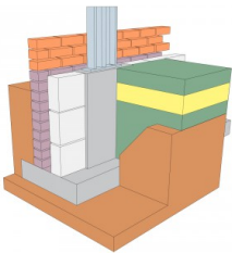
Strip foundations with ground supported floor slab
