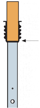
Fig 3b3: Side view. No gap between the bottom of the header and the Steel Strong-Portal shoe
