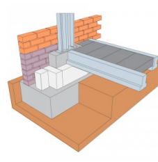
Strip or trench fill foundations with precast concrete beam and block floor
