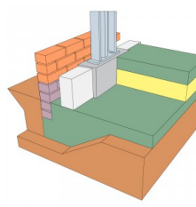
Raft foundations and floor slab
