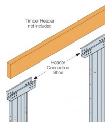
Header connection to shoe. Please note: timber header not included
