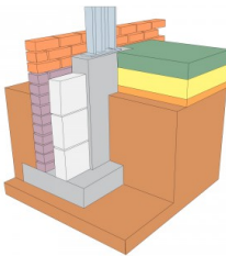
Strip foundations with suspended floor slab
