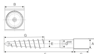
Ground screw fixed technical drawing
