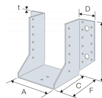
Characteristic capacities - Timber to timber - Full nailing
