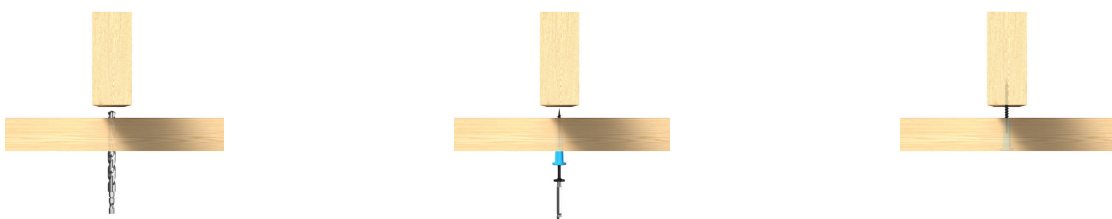
1. Product Choice: For 38 - 47mm top plate with upto 15mm gap - use SDPW14312
