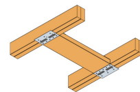
Connecting bracing to double or multiple rafters
