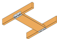
Connecting bracing to single rafters
