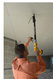
Fixing plasterboard to ceiling.
