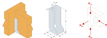
Characteristic capacities - Timber to timber - Partial nailing
