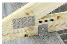
E5 - Fixation bois/support rigide - Appui glissant
